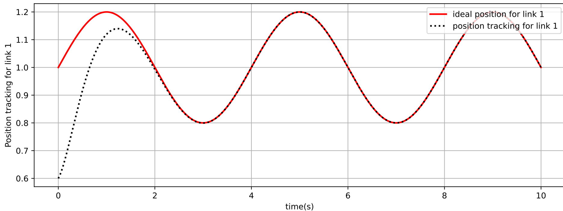
Position Tracking Performance ( S=2 , S1=1 , m=5 )
